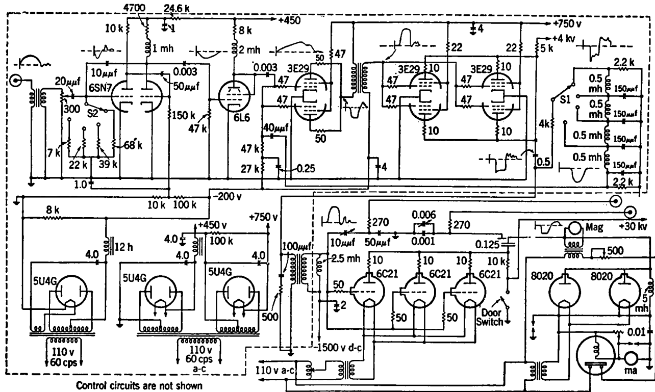
FIG. 5-9.—Schematic diagram for the Model 9 1-Mw hard-tube pulser. Control circuits are not shown.
